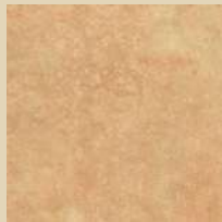
32 Random faces
